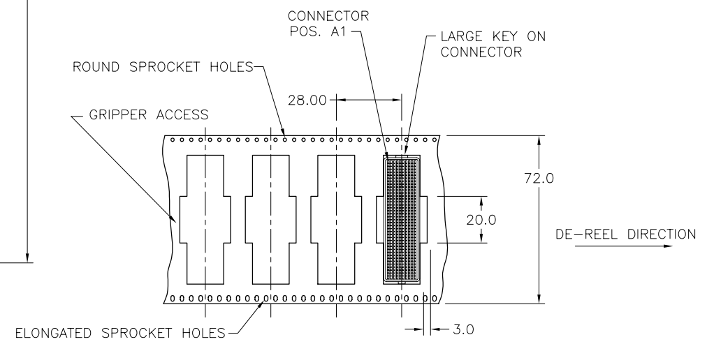
TAPE & REEL PACKAGING SCALE NONE CONFIDENTIAL: INTEL INTERNAL USE ONLY. SEE NOTE 3.
